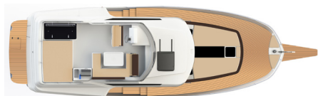
FlyLounge layout
