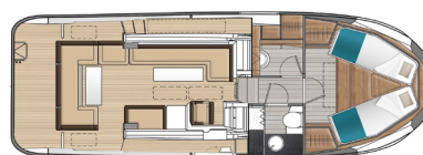
Lower deck - 1 cabin / 1 head
